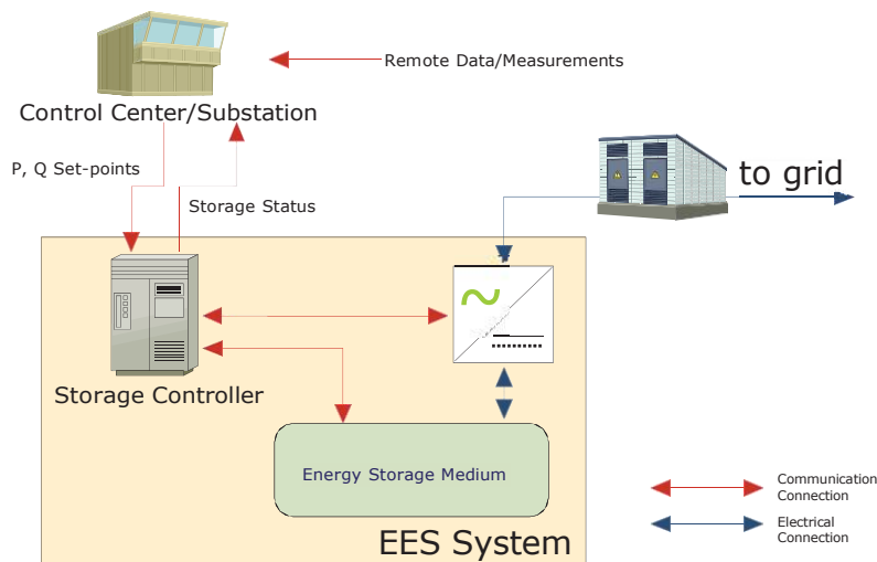
Figure 3-18 | A Control hierarchy involving remote data/measurements (ABB)
