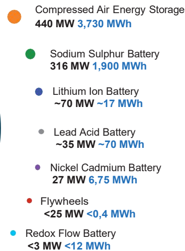
Figure 3-6 | Worldwide installed storage capacity for electrical energy [epri10] [doe07]
