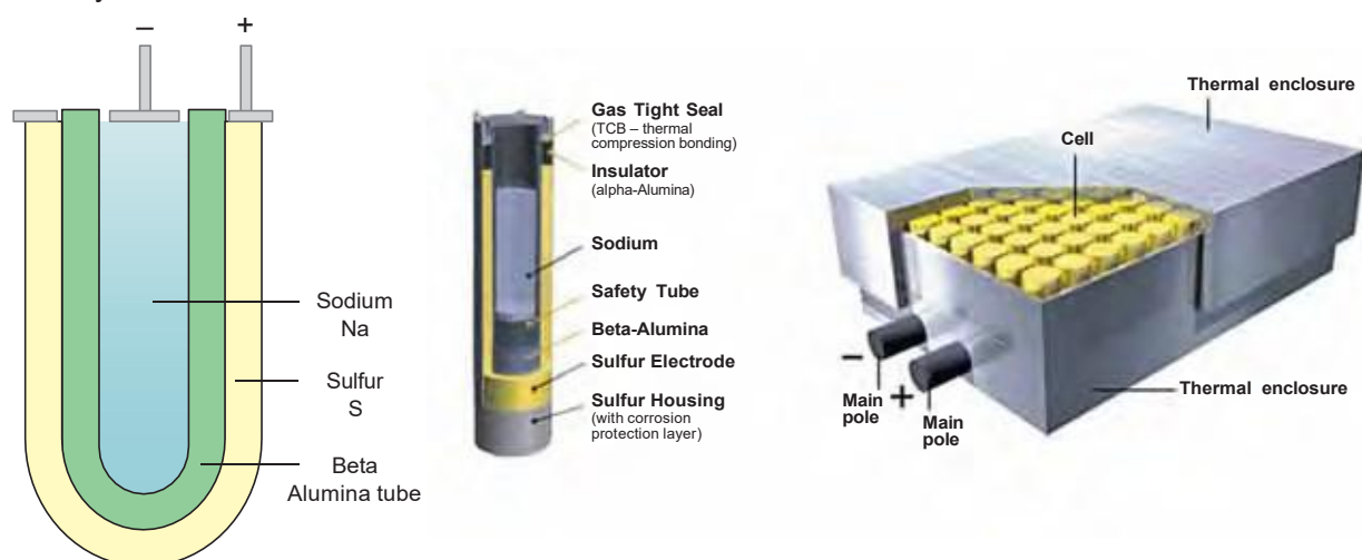
Battery Cell
