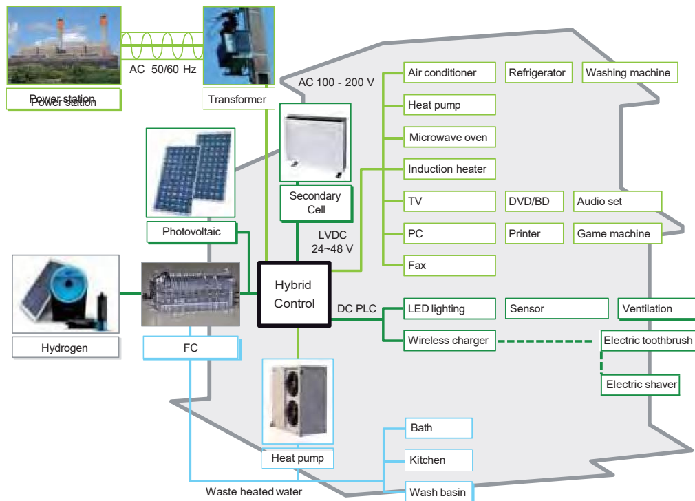
Figure 3-15 | Future home energy network in a smart house (IEC White Paper 2010)
